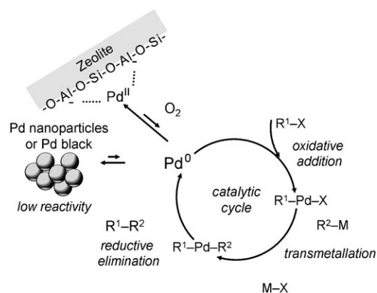
Scheme 1. Proposed reaction mechanism for \text{Pd}^{2+} -exchanged zeolite catalysts under aerobic atmosphere.
