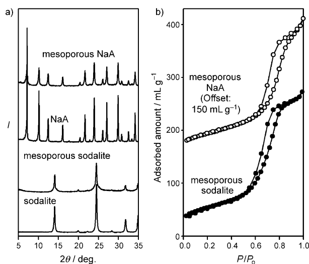
Figure 1. a) XRD patterns and b) N 2 adsorption–desorption isotherms of mesoporous sodalite and NaA zeolite.
